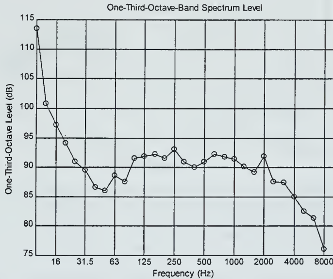
Figure 4.2. One-third-octave-band noise spectrum for the Monterey Bay offshore location.
